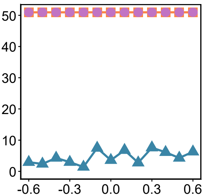
Interest Diversity
