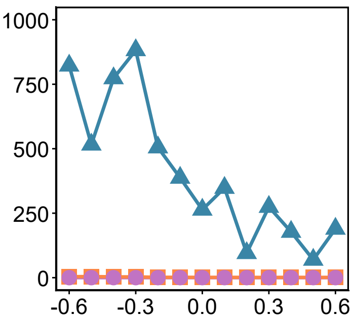
Collective variance
